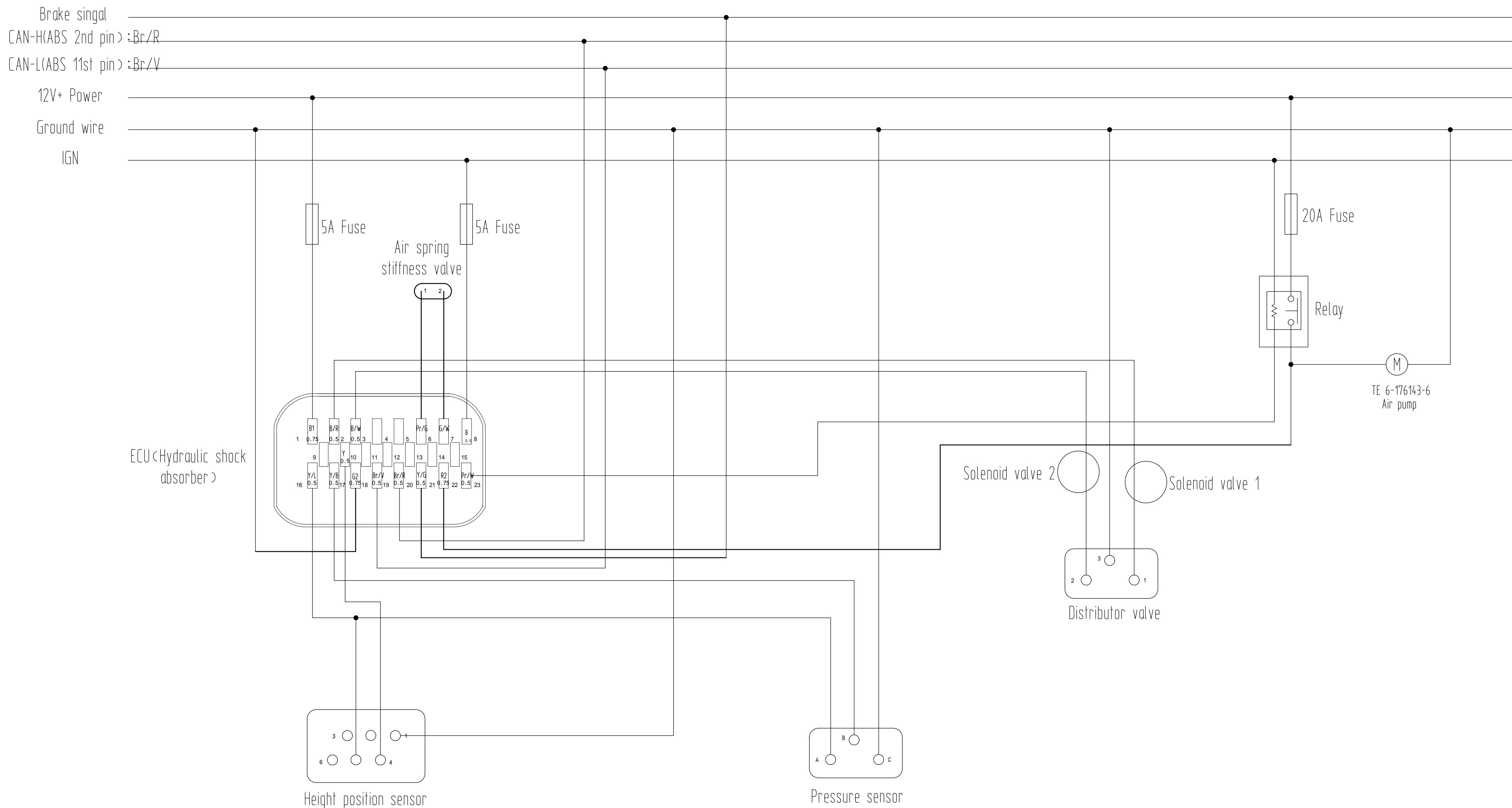
BD700-2A Electric diagram of air shock absorber
